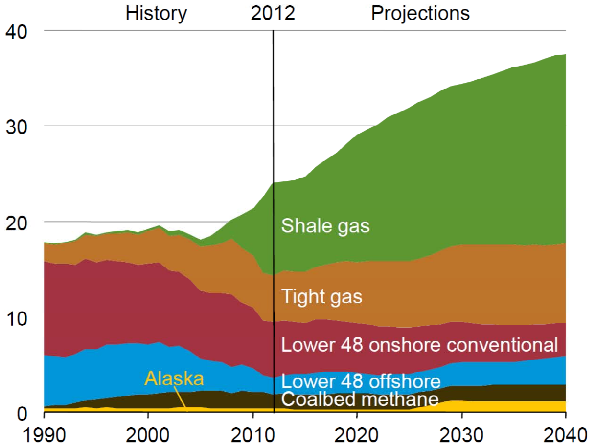
Figure 3.—Projected Domestic Natural Gas Production by Source, 1990-2040 (trillions of cubic feet per day)
